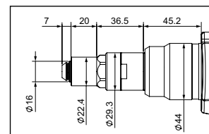
Nose piece access dimensions
